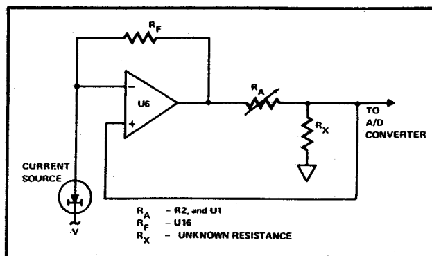
Figure 3-2. Buffer Amplifier for K\Omega Function
