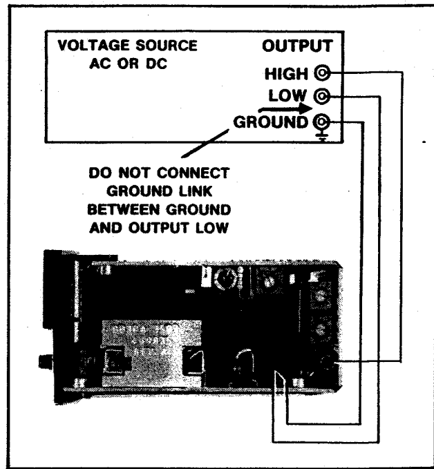
Figure 4-2. Required Method for Voltage Source Connection
