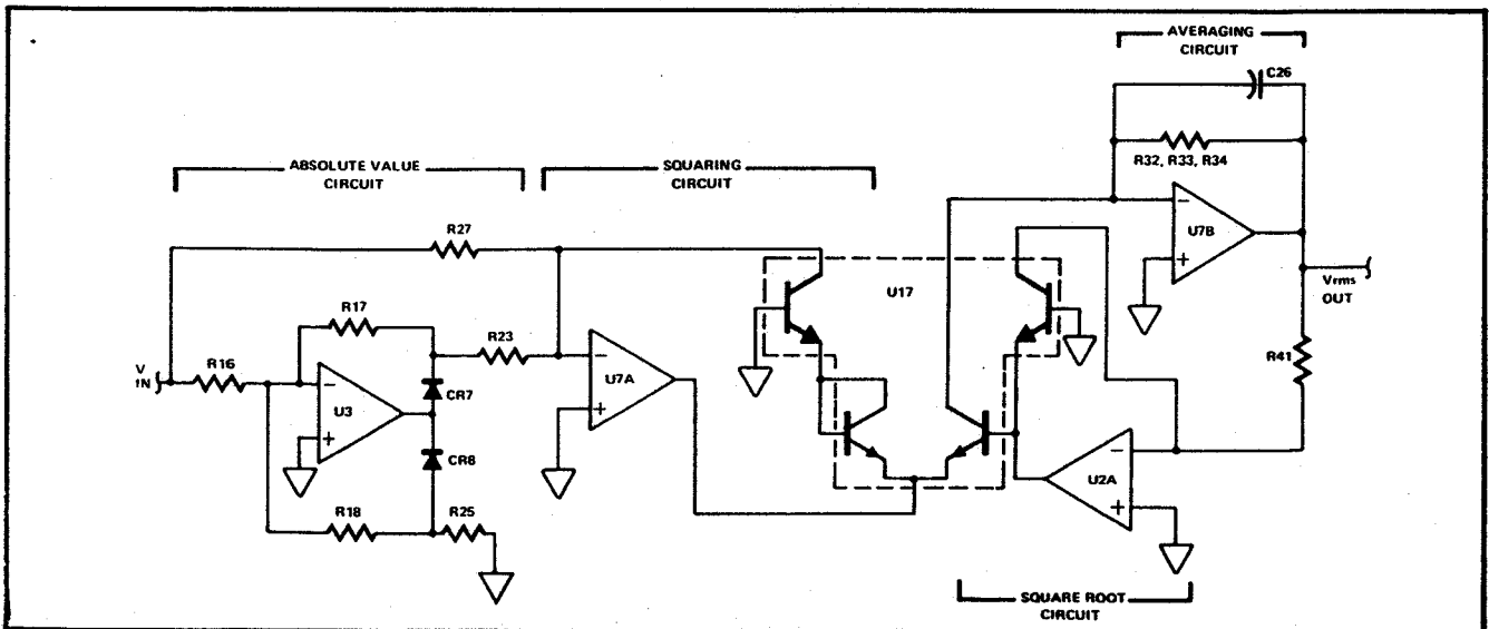
Figure 3-4. True RMS AC Converter
